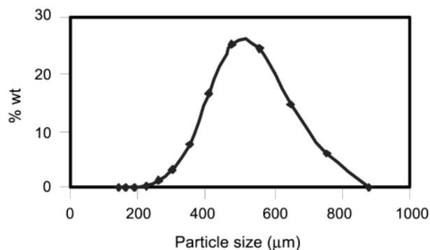
Fig. 2. Glass beads size distribution.
