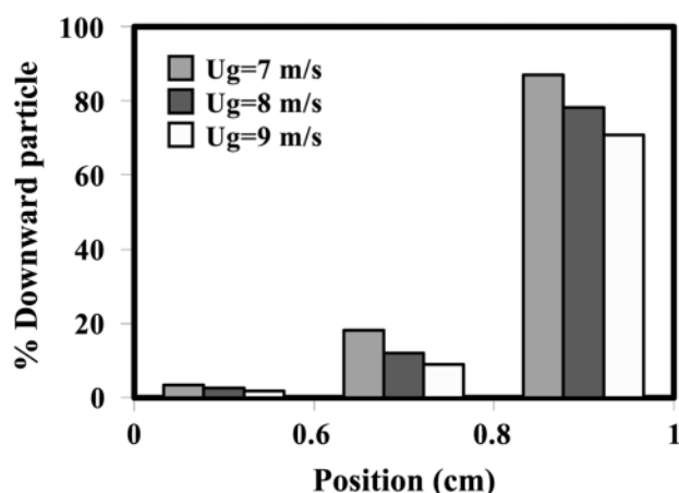
Fig. 9. Particle holdup moving downward as a function of radial position at different U_g and 110 cm high from distributor.
